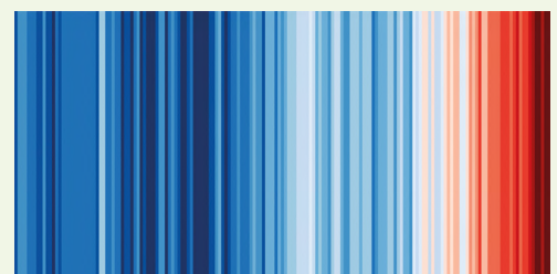
Warming Stripes global 1850 -2020
